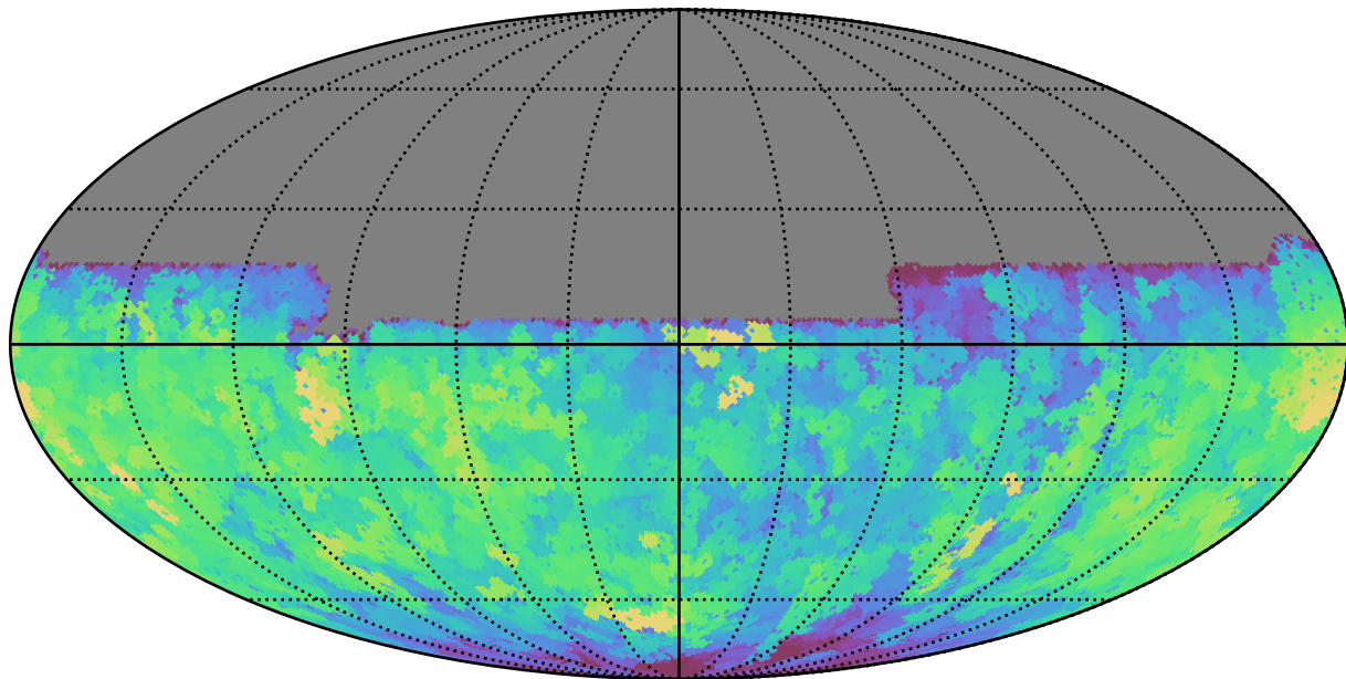
too_5_4v3.4_10yrs All sky u band: Max saturation_mag
