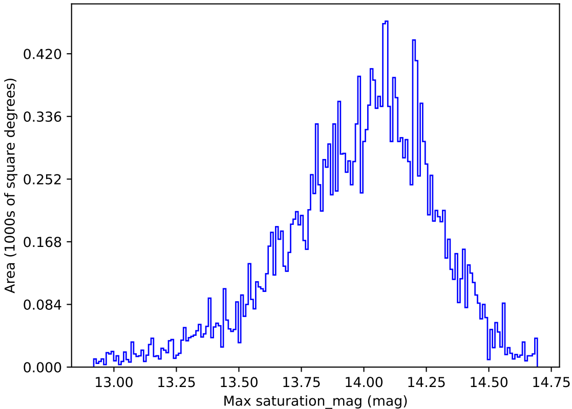
too_5_4v3.4_10yrs All sky u band: Max saturation_mag
