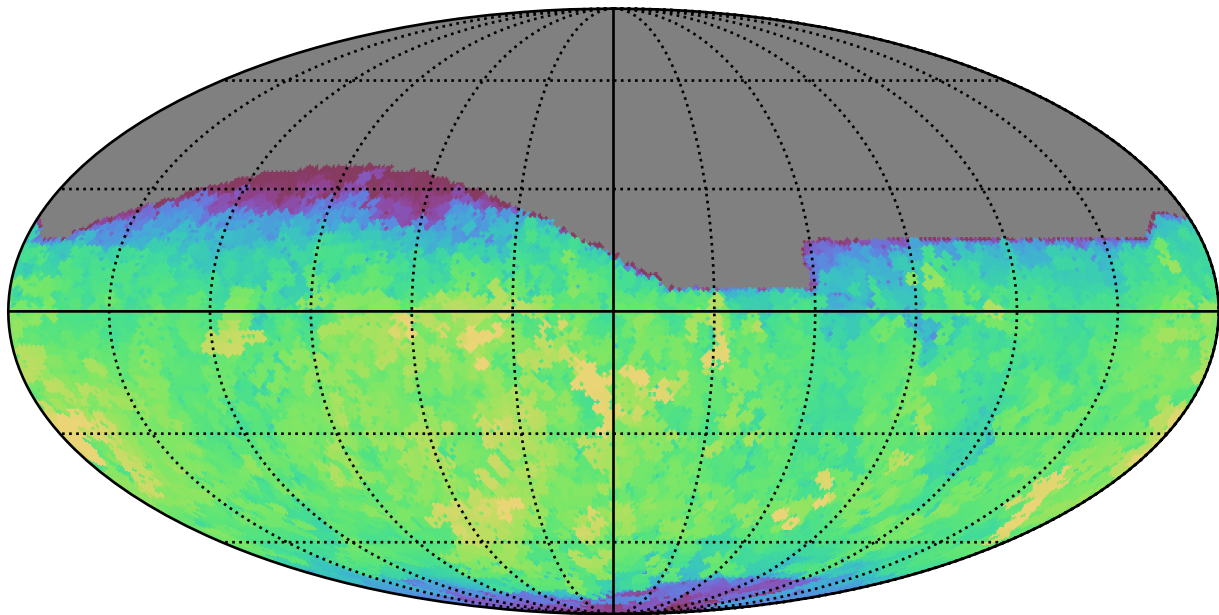
too_5_4v3.4_10yrs All sky r band: Max saturation_mag
