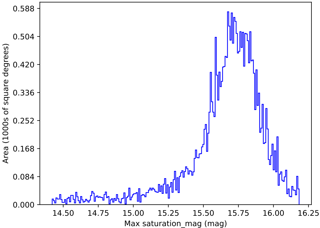
too_5_4v3.4_10yrs All sky r band: Max saturation_mag
