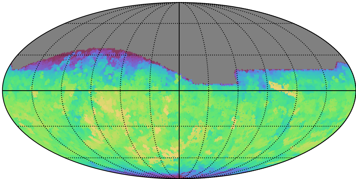
too_5_4v3.4_10yrs All sky i band: Max saturation_mag
