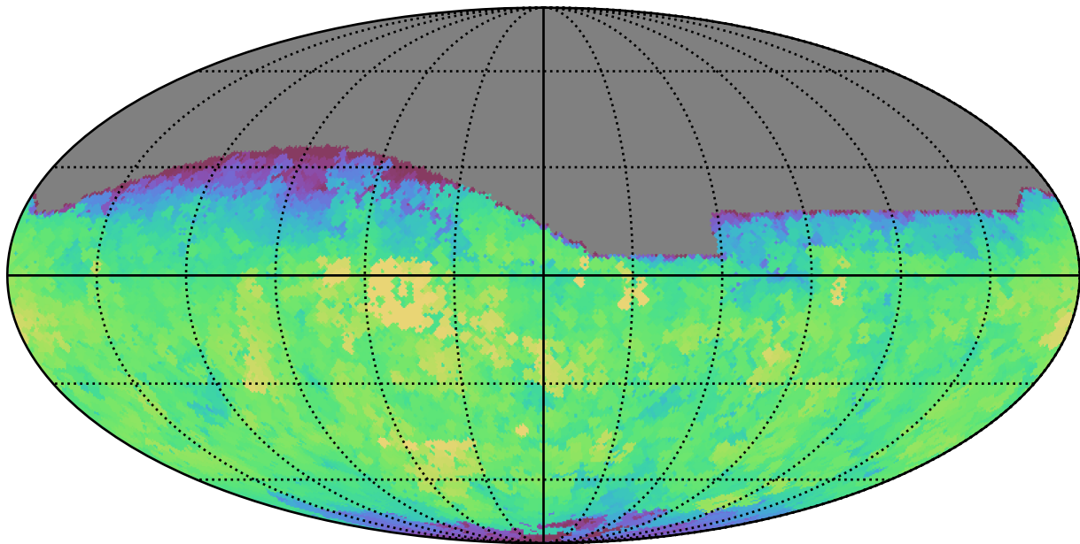
too_5_4v3.4_10yrs All sky g band: Max saturation_mag
