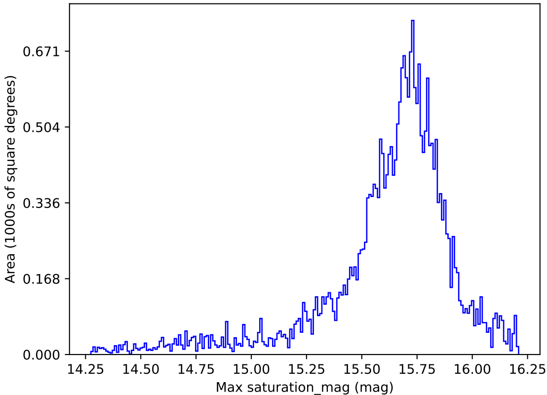
too_5_4v3.4_10yrs All sky g band: Max saturation_mag
