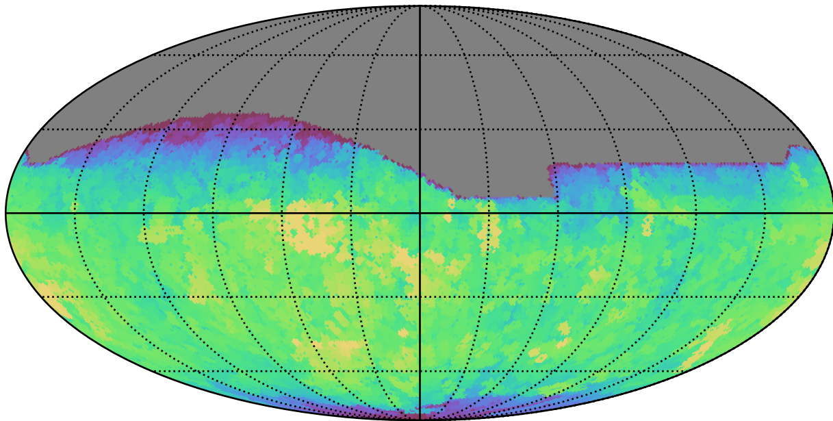
too_5_4v3.4_10yrs All sky all bands: Max saturation_mag
