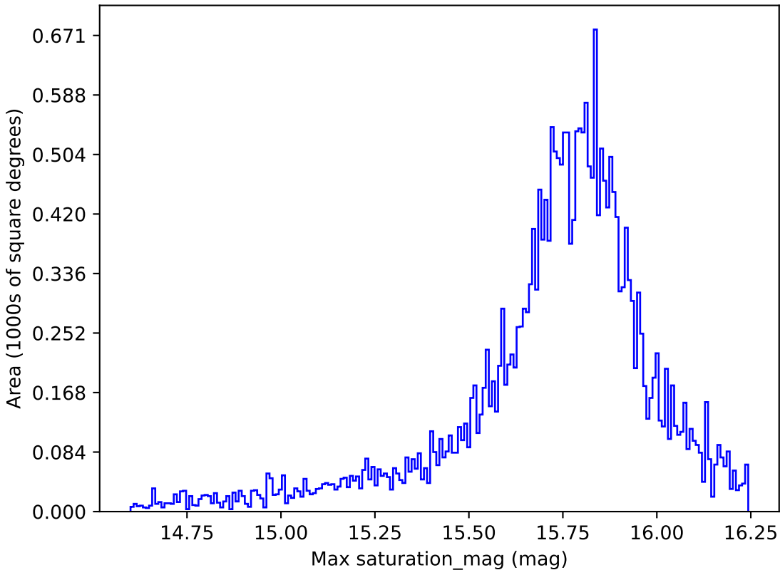
too_5_4v3.4_10yrs All sky all bands: Max saturation_mag
