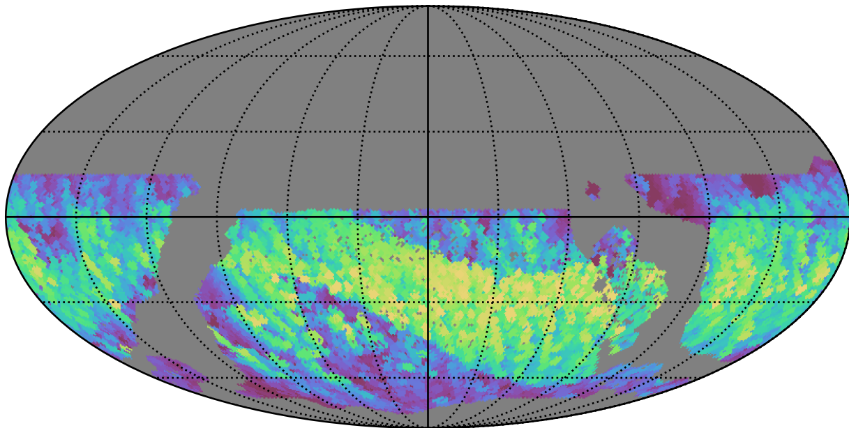
too_5_4v3.4_10yrs WFD z band: Max normairmass
