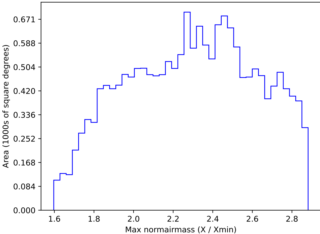
too_5_4v3.4_10yrs WFD z band: Max normairmass
