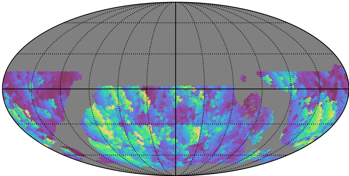
too_5_4v3.4_10yrs WFD u band: Max normairmass
