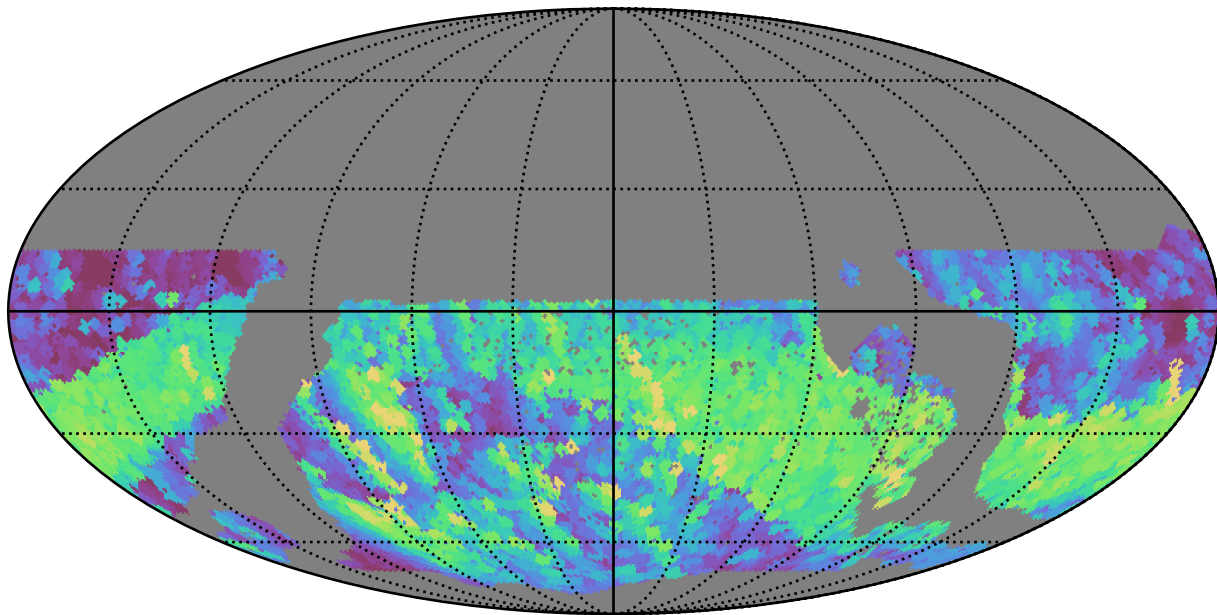
too_5_4v3.4_10yrs WFD r band: Max normairmass
