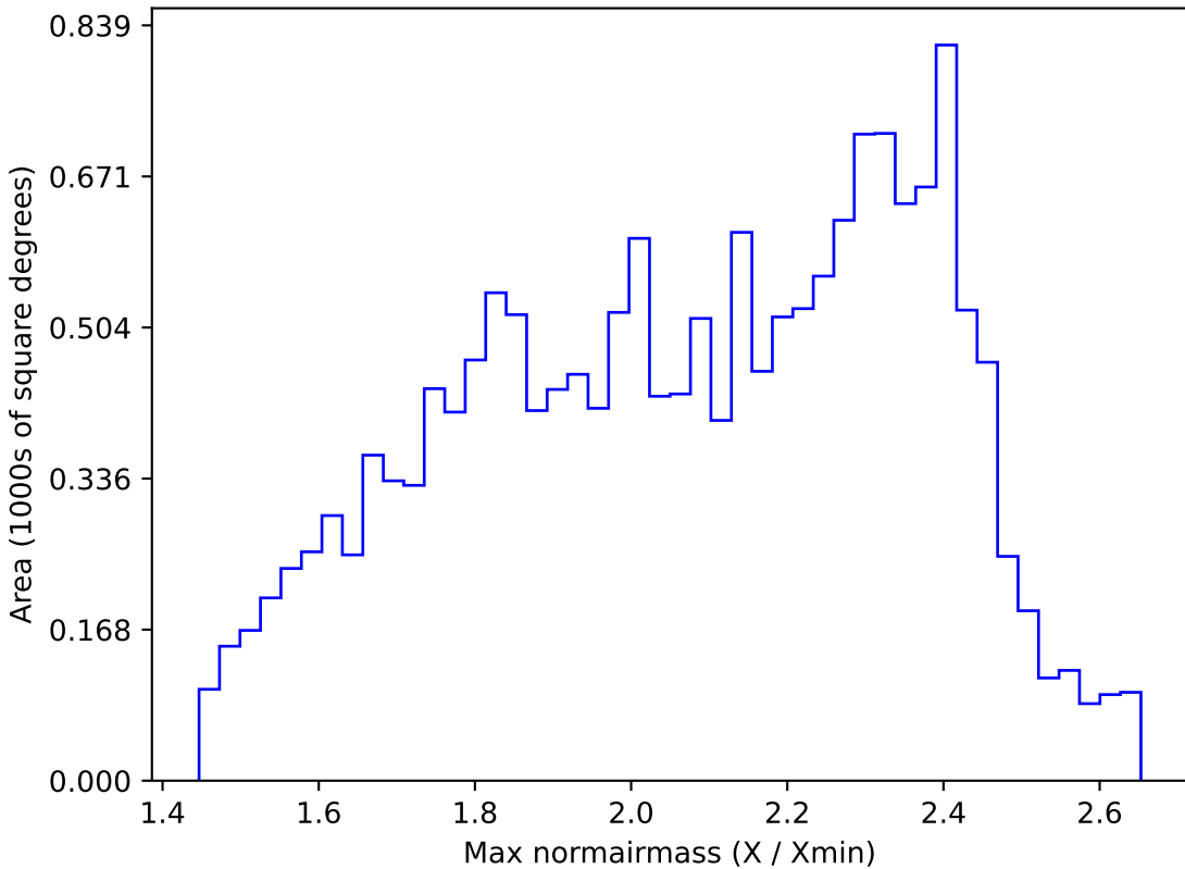
too_5_4v3.4_10yrs WFD r band: Max normairmass
