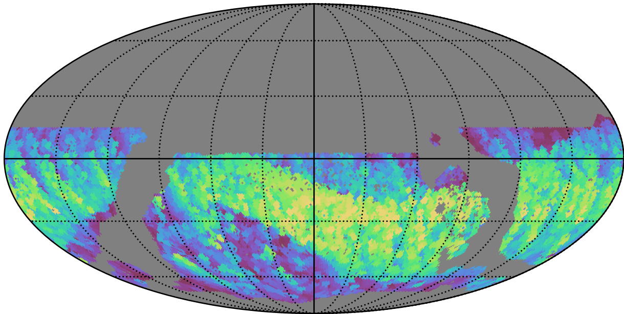
too_5_4v3.4_10yrs WFD i band: Max normairmass
