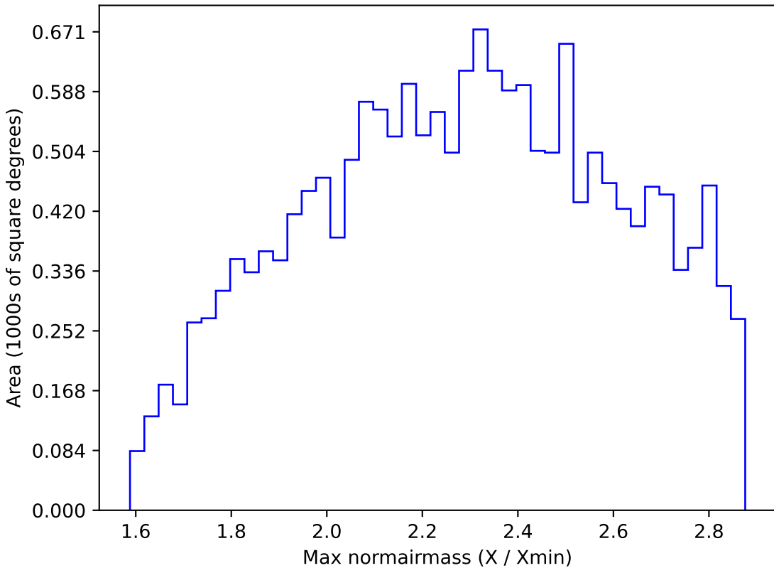
too_5_4v3.4_10yrs WFD i band: Max normairmass
