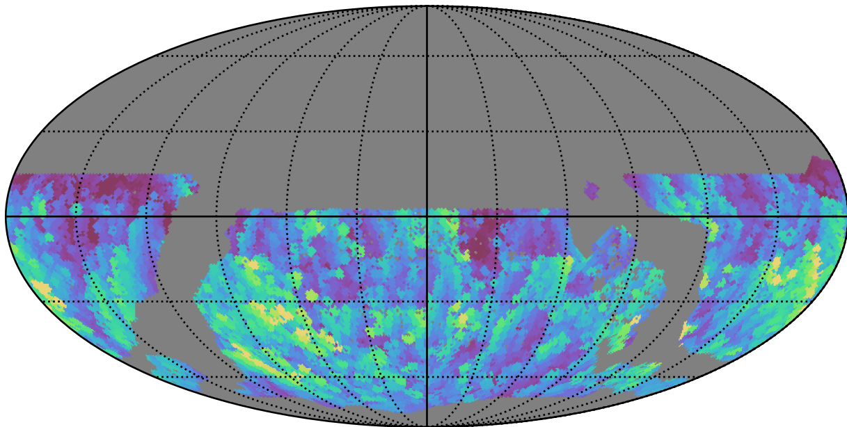
too_5_4v3.4_10yrs WFD g band: Max normairmass
