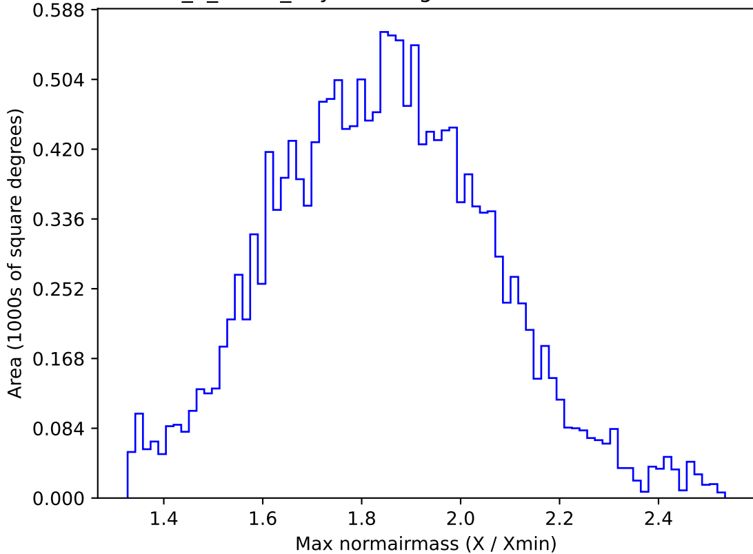
too_5_4v3.4_10yrs WFD g band: Max normairmass
