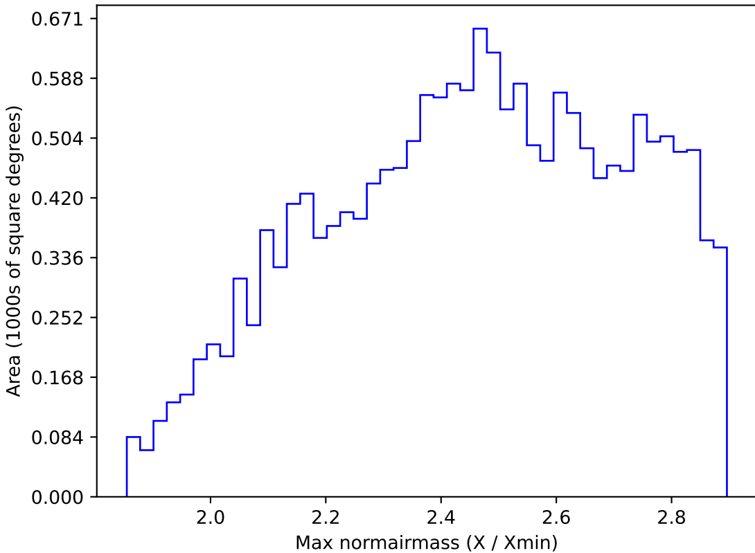
too_5_4v3.4_10yrs WFD all bands: Max normairmass
