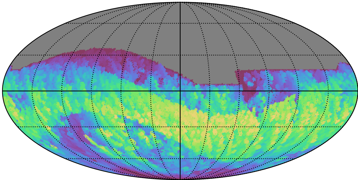
too_5_4v3.4_10yrs All sky z band: Max normairmass
