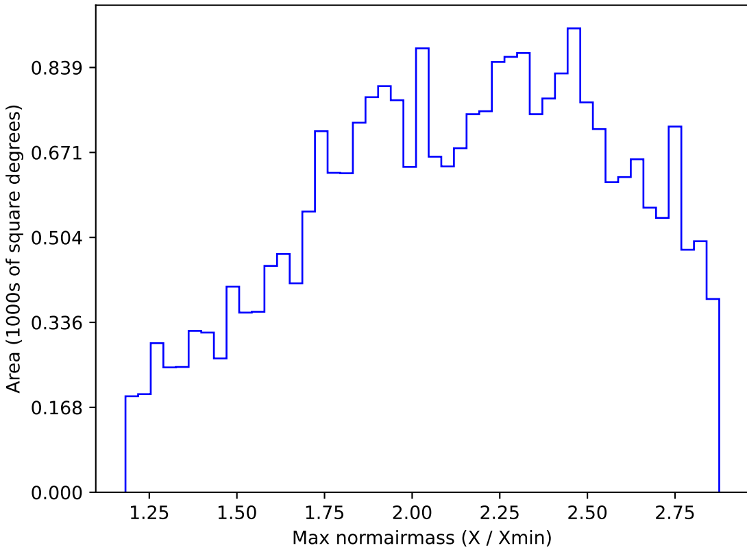
too_5_4v3.4_10yrs All sky z band: Max normairmass
