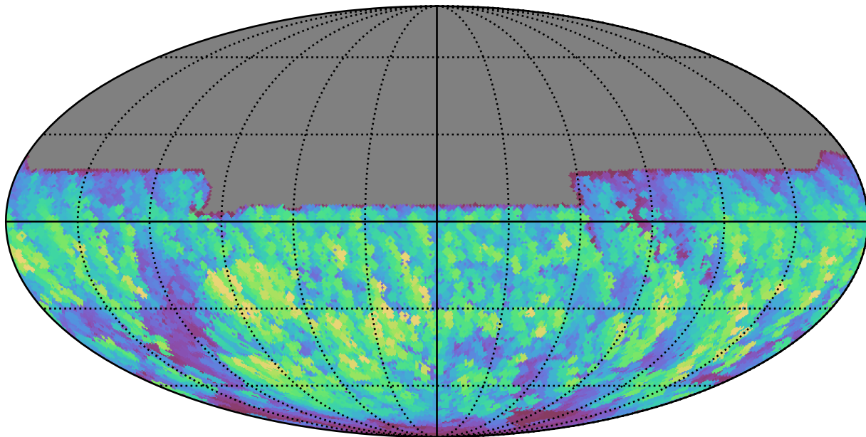
too_5_4v3.4_10yrs All sky y band: Max normairmass
