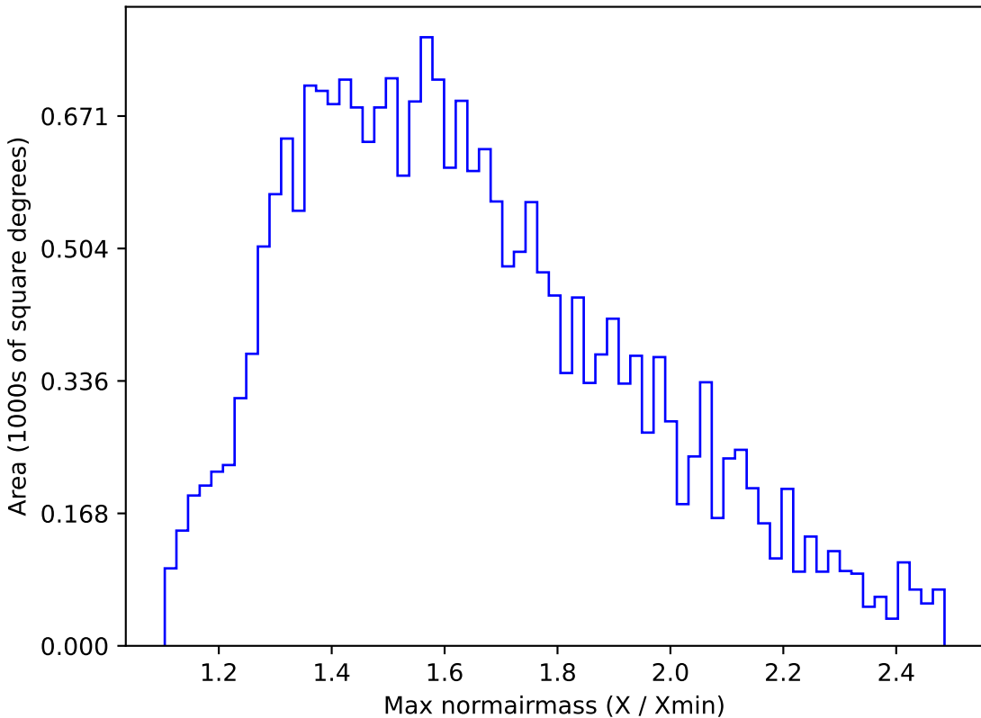
too_5_4v3.4_10yrs All sky u band: Max normairmass
