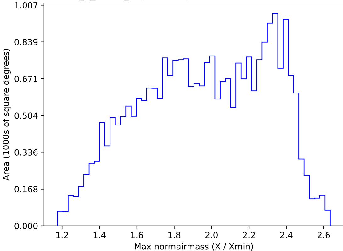
too_5_4v3.4_10yrs All sky r band: Max normairmass
