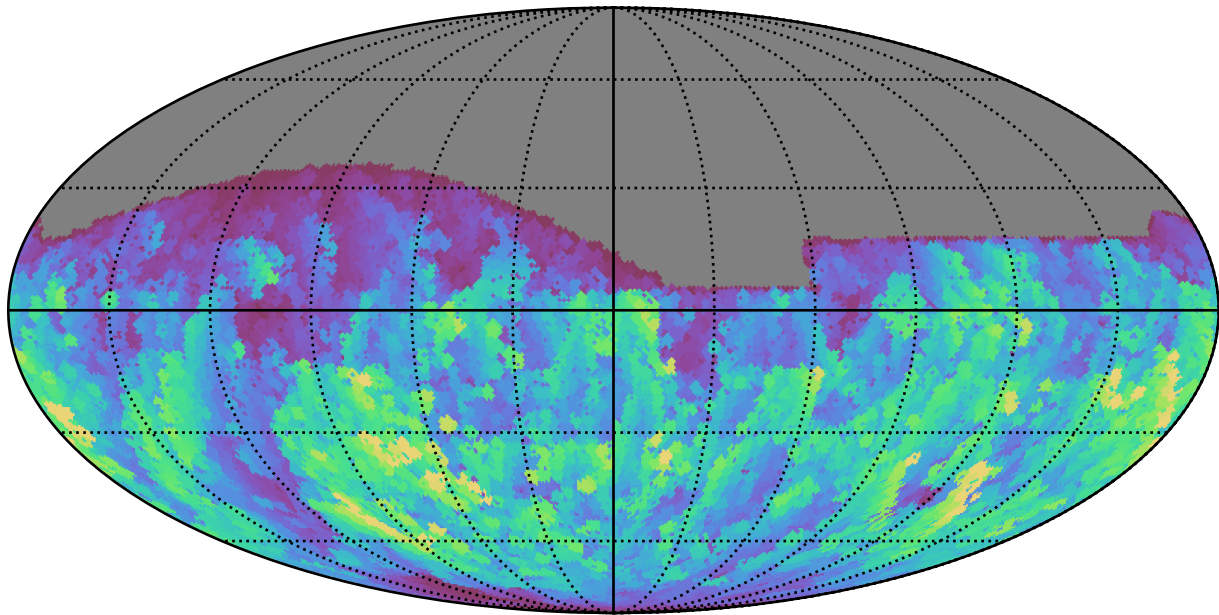
too_5_4v3.4_10yrs All sky g band: Max normairmass
