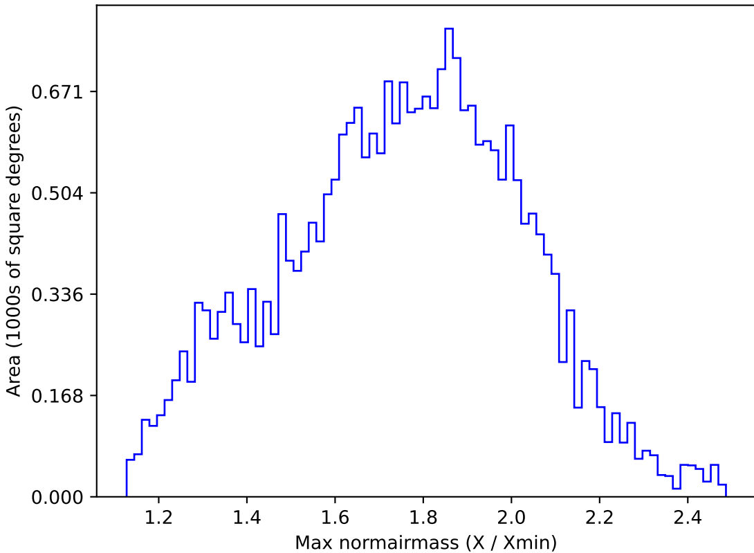
too_5_4v3.4_10yrs All sky g band: Max normairmass
