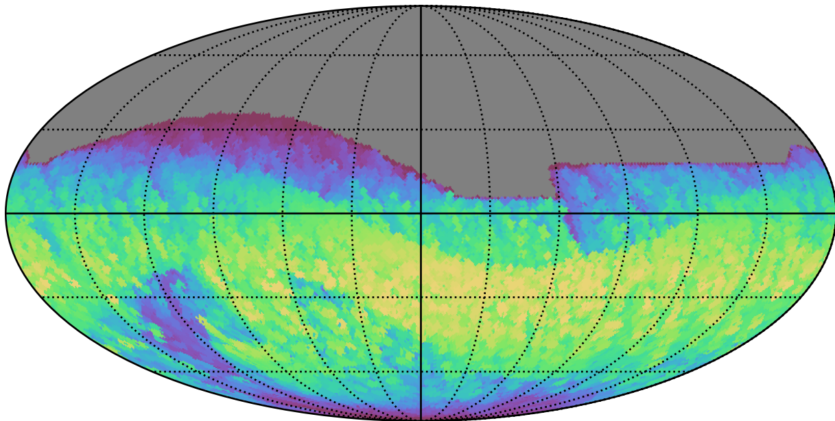
too_5_4v3.4_10yrs All sky all bands: Max normairmass
