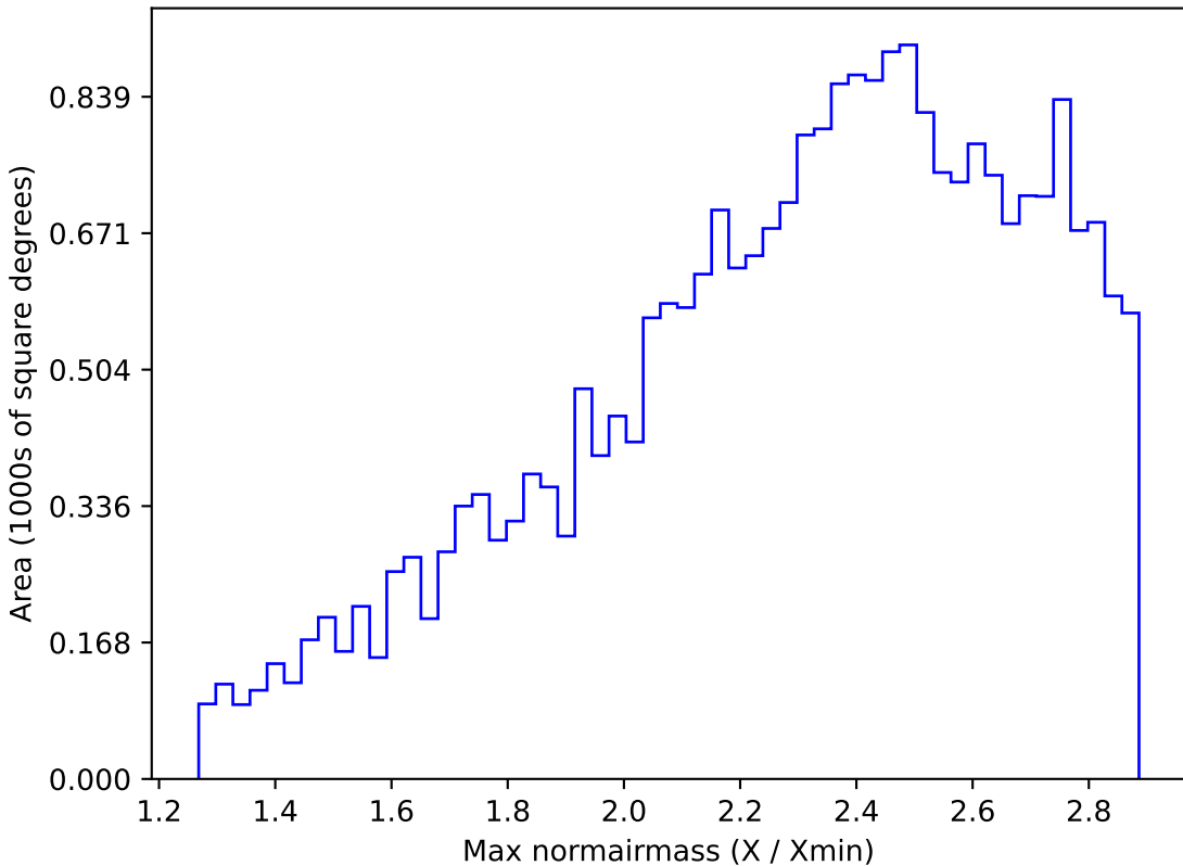
too_5_4v3.4_10yrs All sky all bands: Max normairmass
