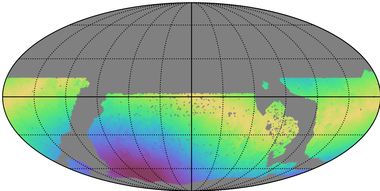
too_5_4v3.4_10yrs WFD z band: Max moonDistance
