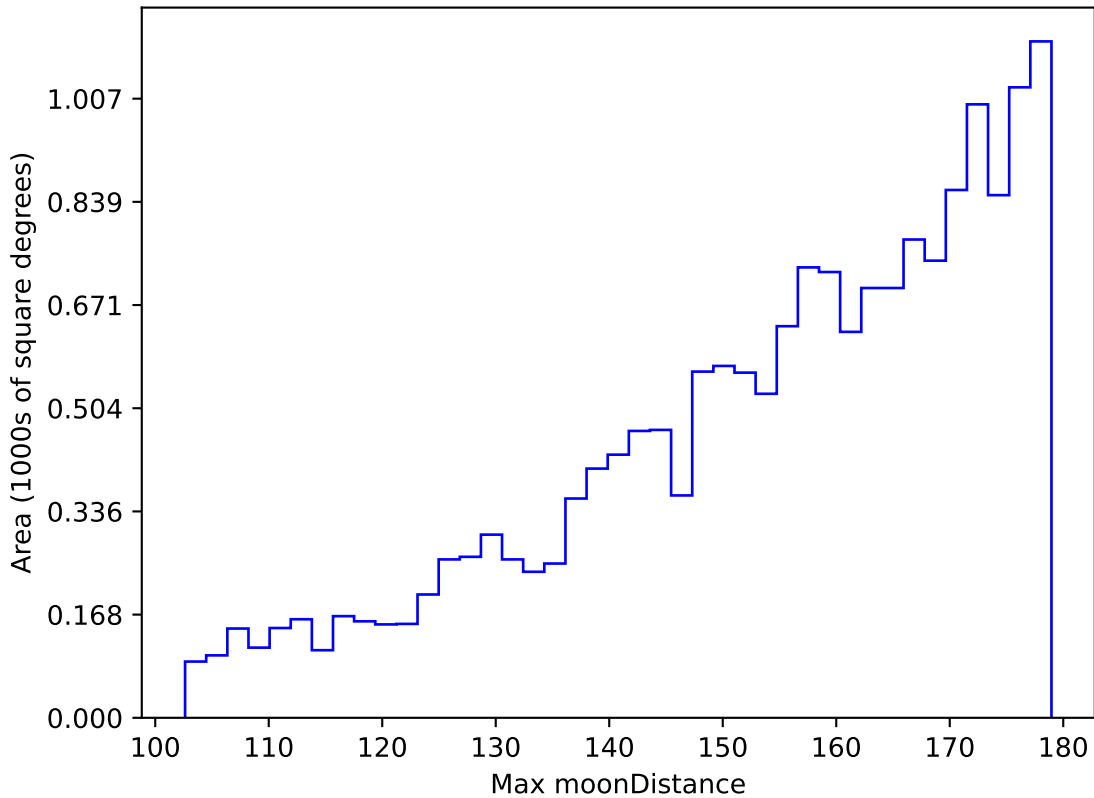
too_5_4v3.4_10yrs WFD z band: Max moonDistance
