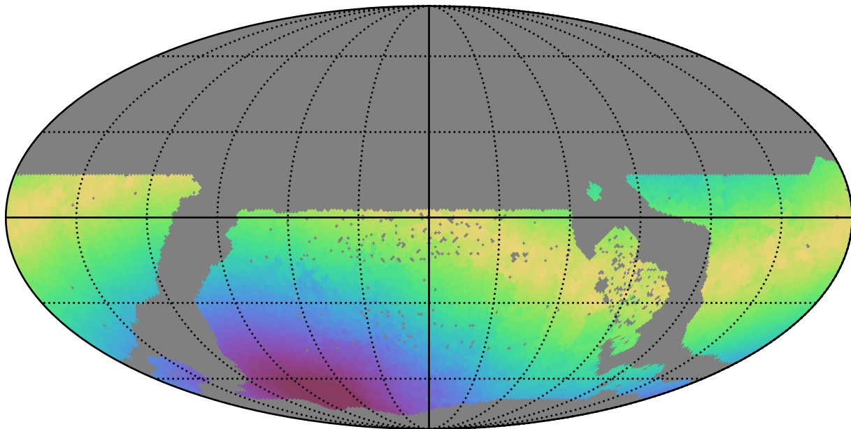
too_5_4v3.4_10yrs WFD u band: Max moonDistance
