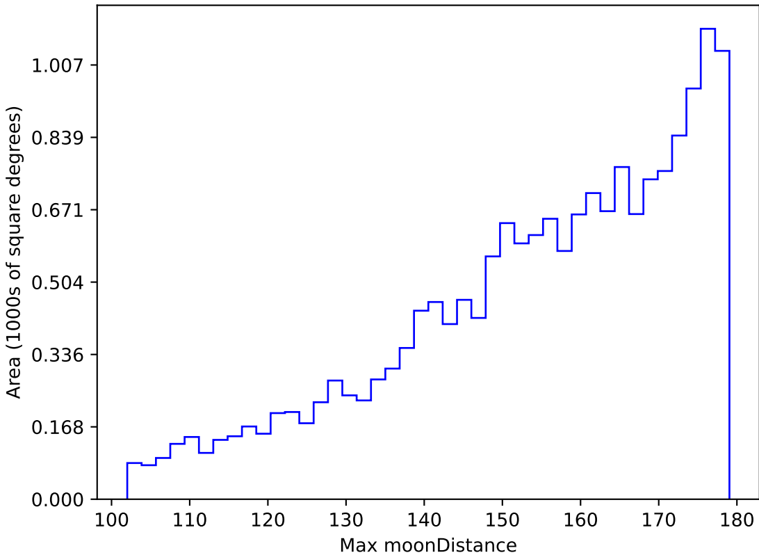
too_5_4v3.4_10yrs WFD u band: Max moonDistance
