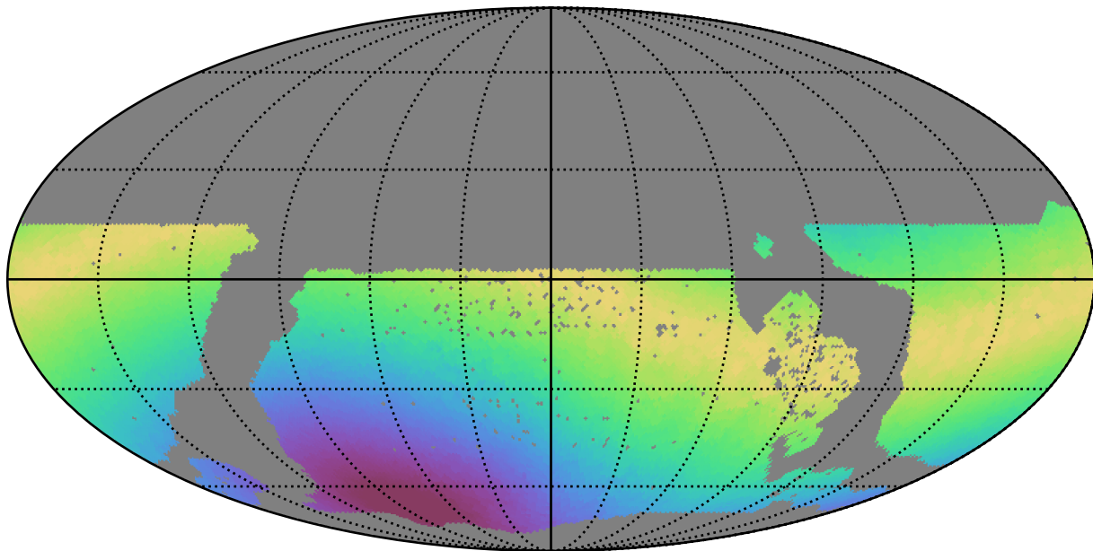
too_5_4v3.4_10yrs WFD r band: Max moonDistance
