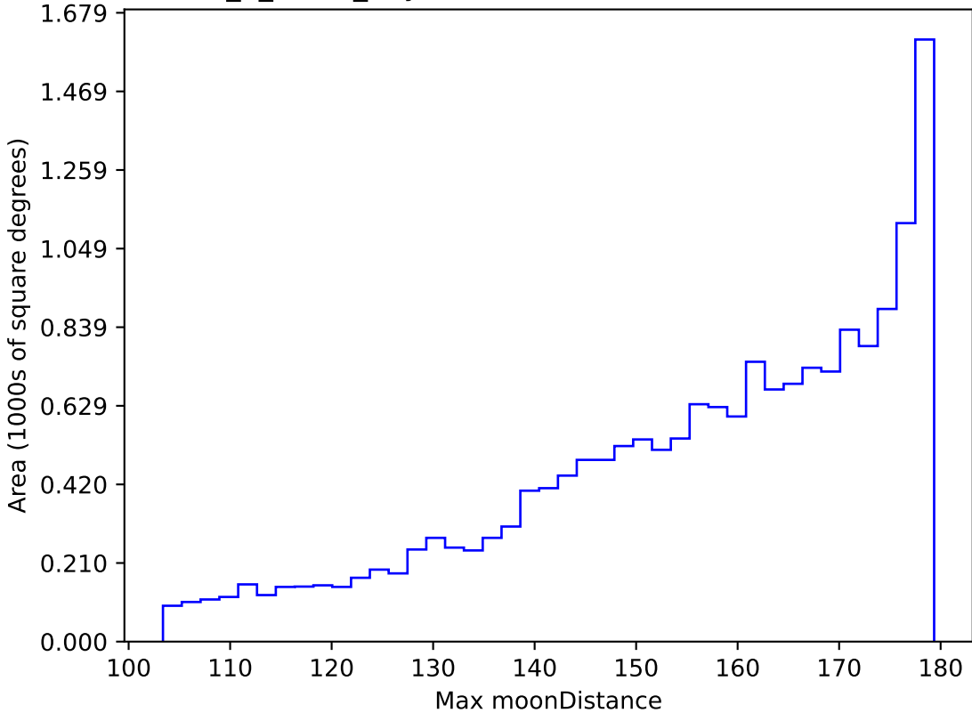
too_5_4v3.4_10yrs WFD r band: Max moonDistance
