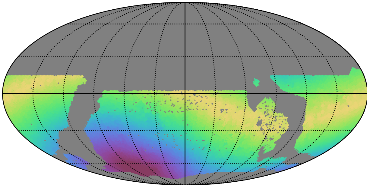
too_5_4v3.4_10yrs WFD i band: Max moonDistance
