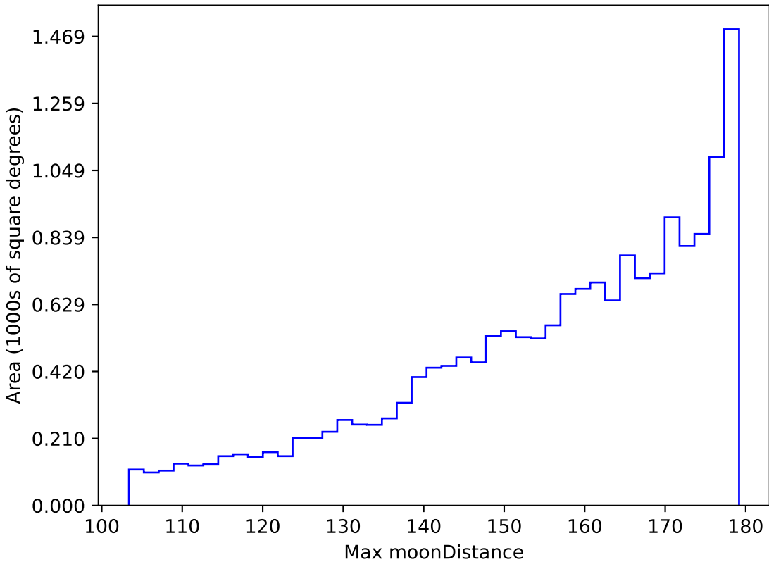
too_5_4v3.4_10yrs WFD i band: Max moonDistance
