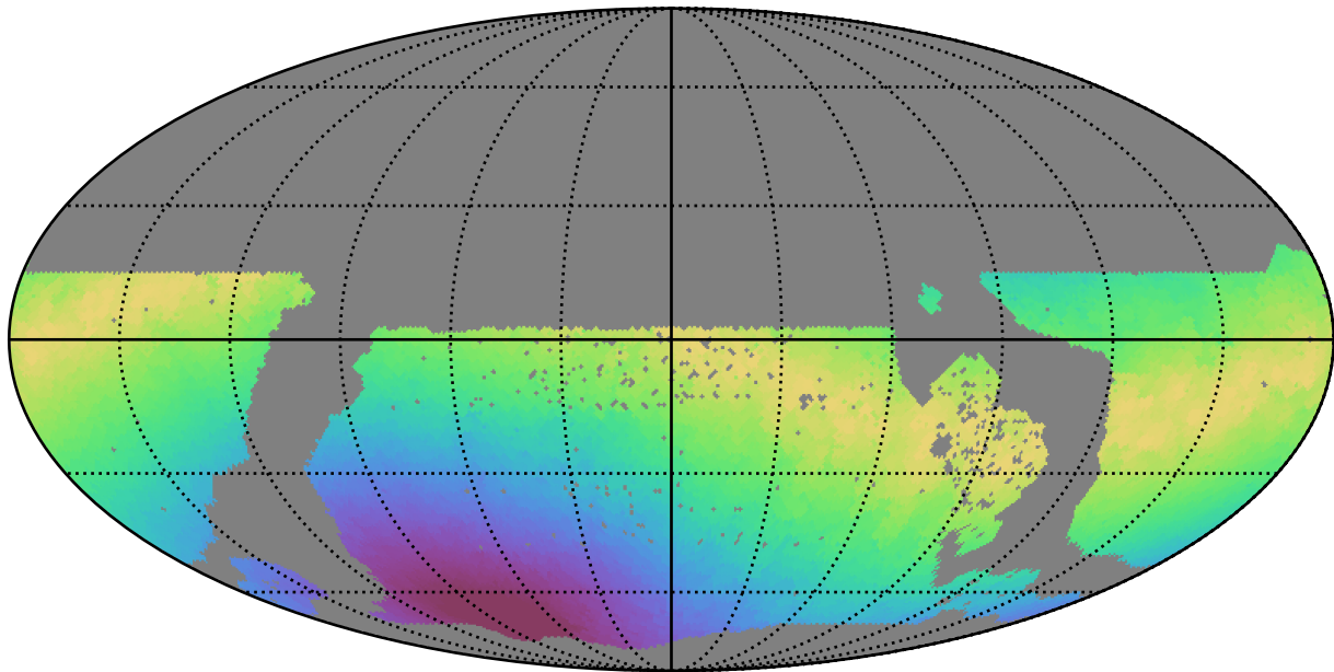
too_5_4v3.4_10yrs WFD g band: Max moonDistance
