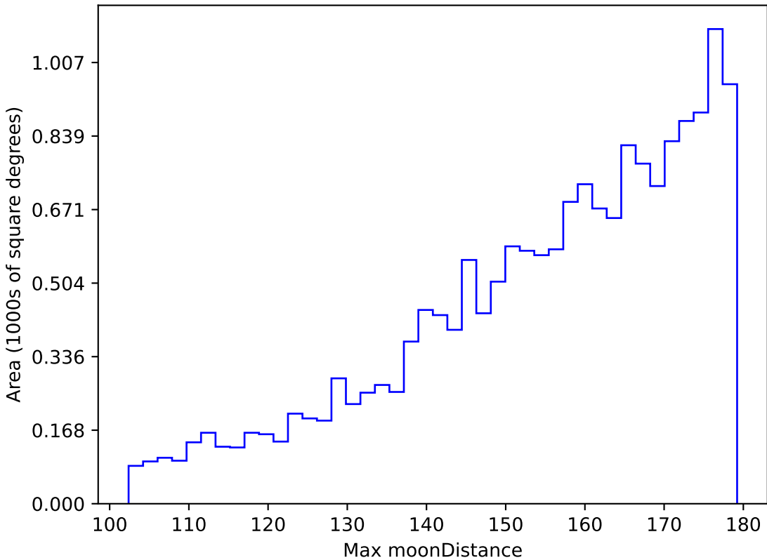
too_5_4v3.4_10yrs WFD g band: Max moonDistance
