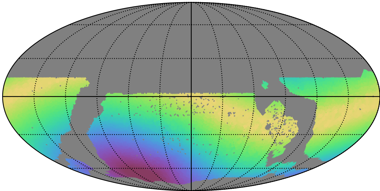
too_5_4v3.4_10yrs WFD all bands: Max moonDistance
