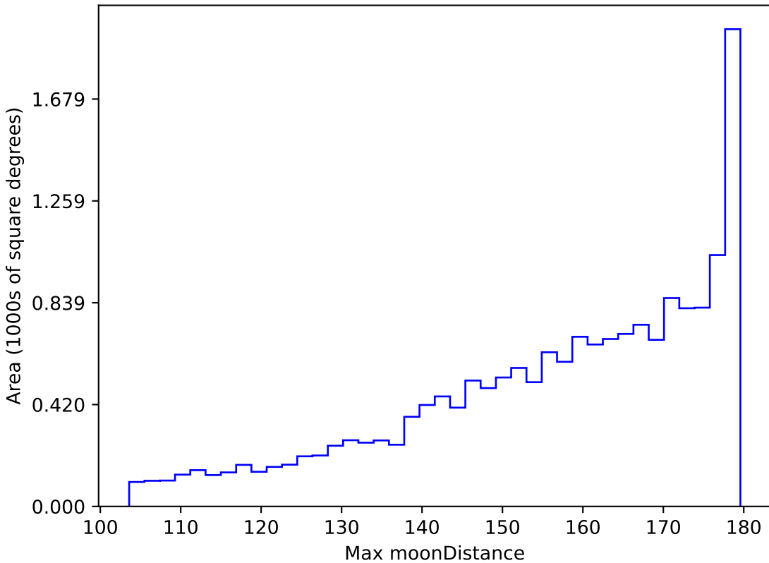
too_5_4v3.4_10yrs WFD all bands: Max moonDistance
