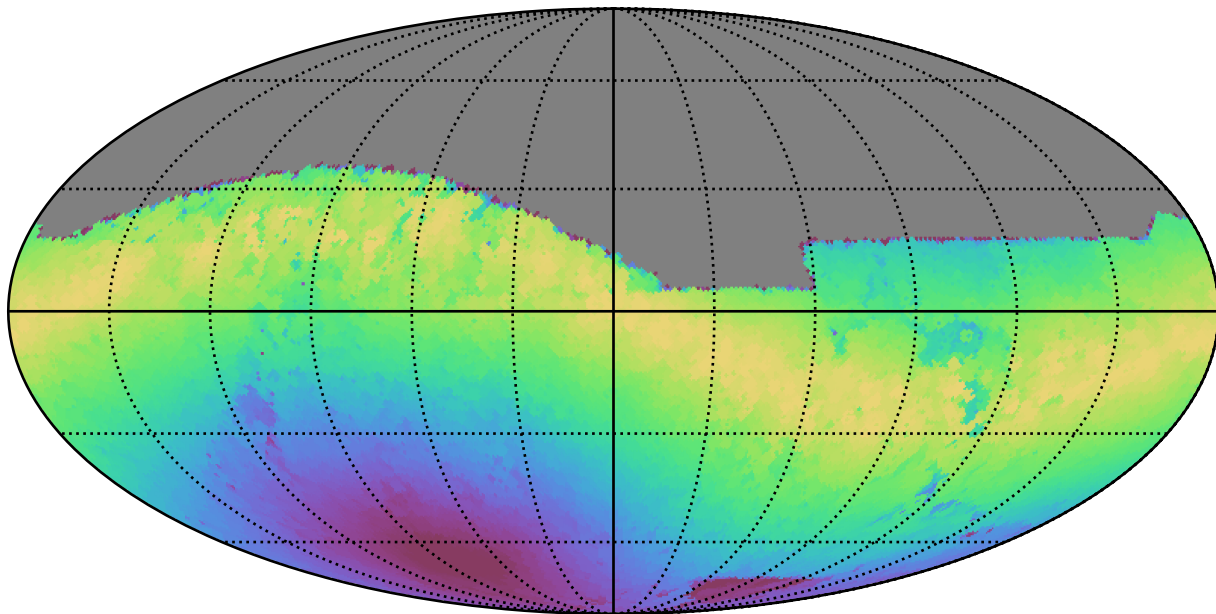
too_5_4v3.4_10yrs All sky z band: Max moonDistance
