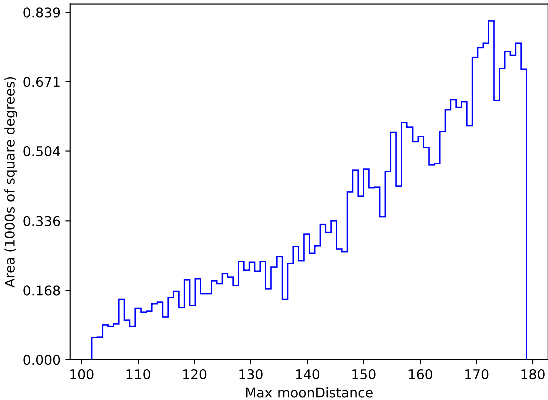
too_5_4v3.4_10yrs All sky z band: Max moonDistance
