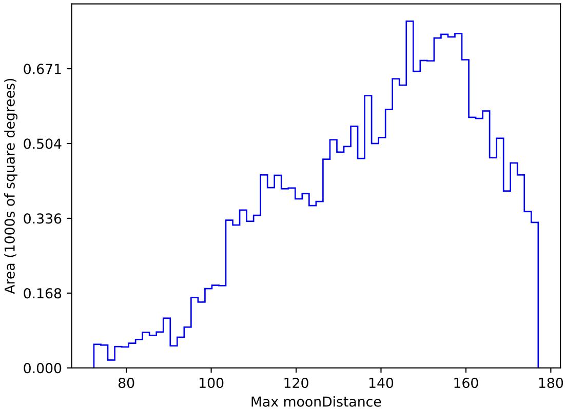
too_5_4v3.4_10yrs All sky y band: Max moonDistance
