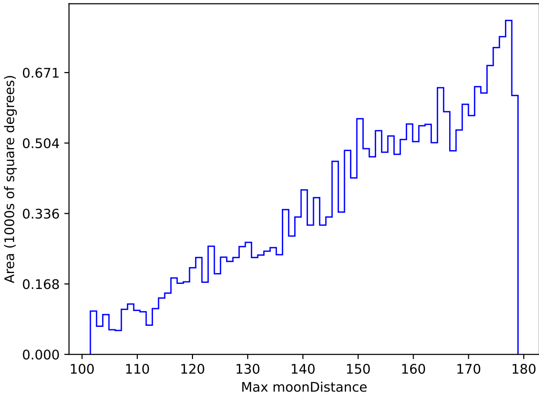
too_5_4v3.4_10yrs All sky u band: Max moonDistance
