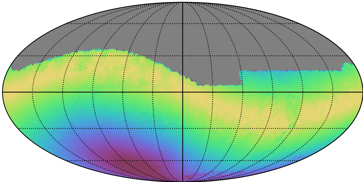
too_5_4v3.4_10yrs All sky r band: Max moonDistance
