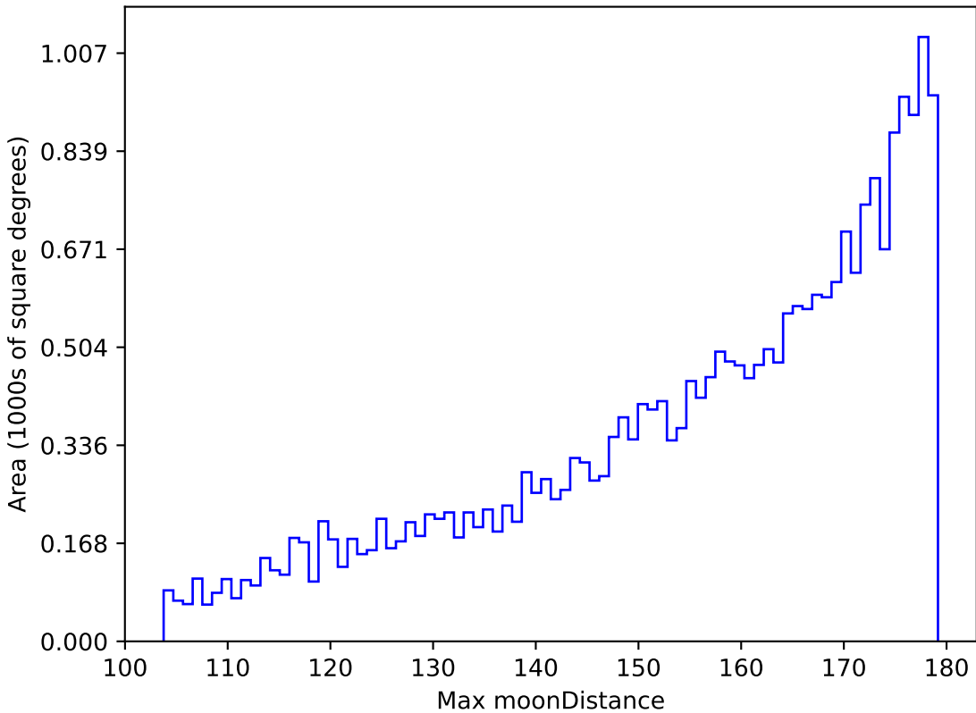
too_5_4v3.4_10yrs All sky i band: Max moonDistance
