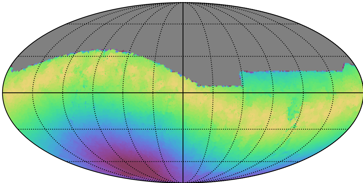
too_5_4v3.4_10yrs All sky g band: Max moonDistance
