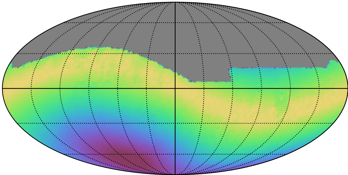
too_5_4v3.4_10yrs All sky all bands: Max moonDistance
