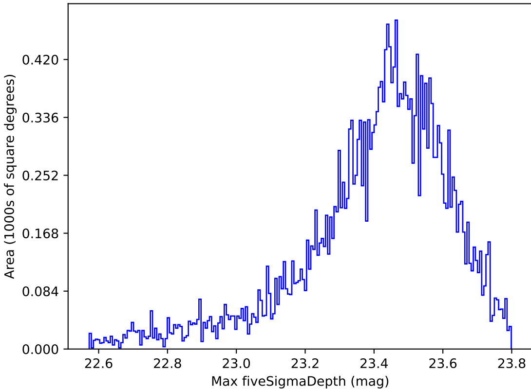
too_5_4v3.4_10yrs Yr 1 z band: Max fiveSigmaDepth
