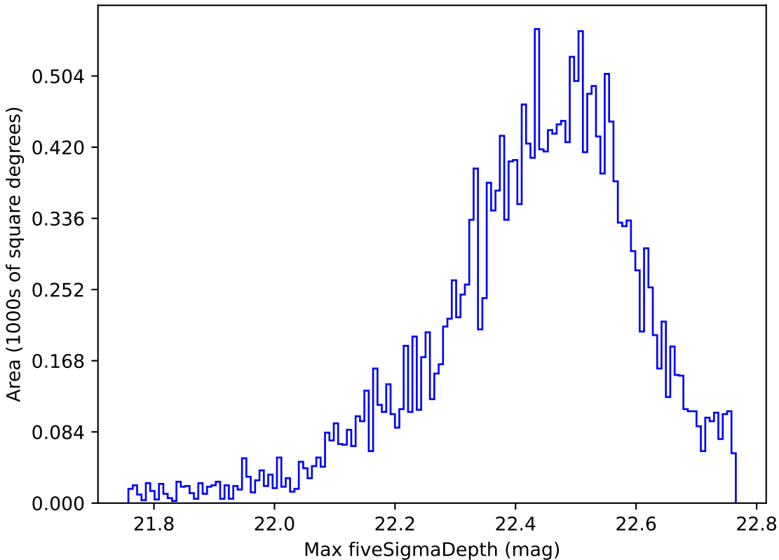
too_5_4v3.4_10yrs Yr 1 y band: Max fiveSigmaDepth
